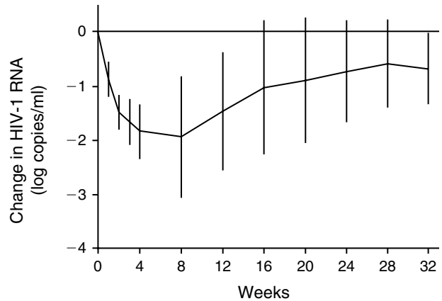
Figure 3. Changes from Base Line in the Mean ( \pm SD) Concentration of HIV-1 RNA as Measured by a More Sensitive PCR Assay in 17 Consecutive Patients in the Subgroups Receiving 500 mg and 600 mg of Ritonavir Every 12 Hours during the Maintenance Phase, Lasting up to 32 Weeks.
