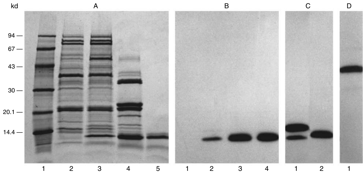
Figure 2. Results of SDS-PAGE and Autoradiography.
