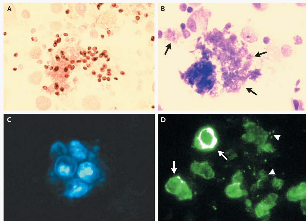
Figure 2. Detection of Pneumocystis Forms with the Use of Different Stains.
