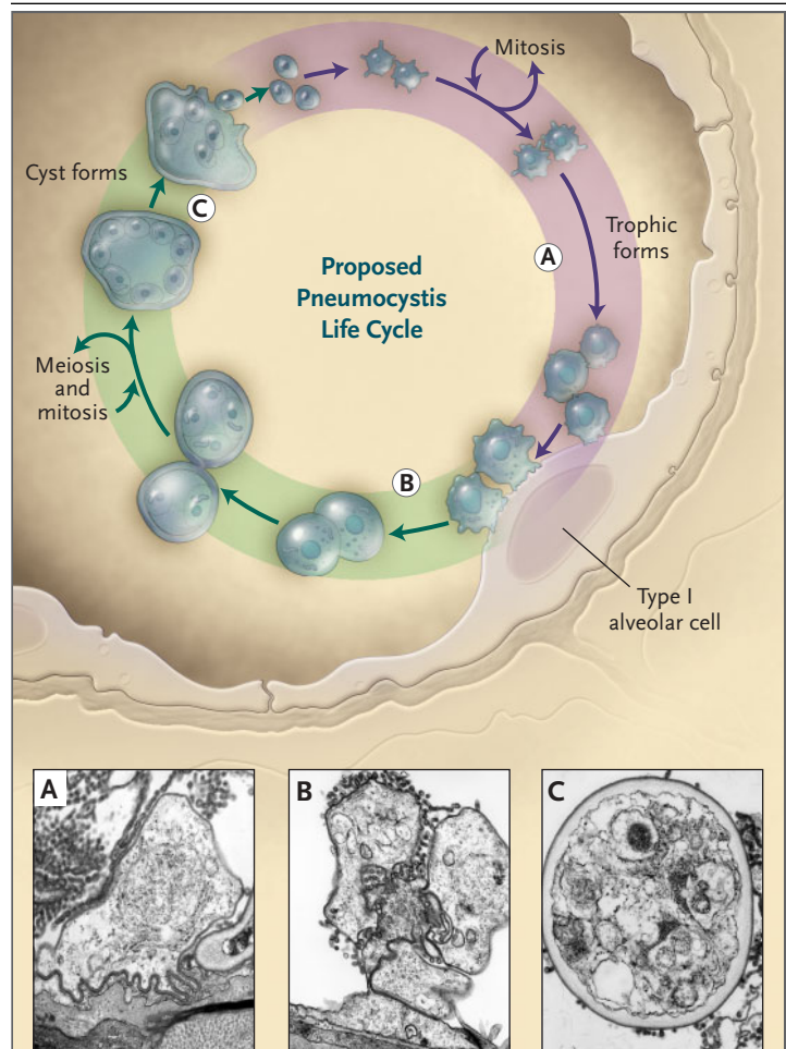
Figure 3. Proposed Pneumocystis Life Cycle.
