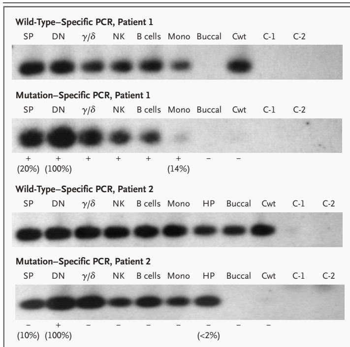
Figure 2. Hybridization of the PCR Products of Fas Exon 8 after Wild-Type-Specific and Mutation-Specific Amplifications.
